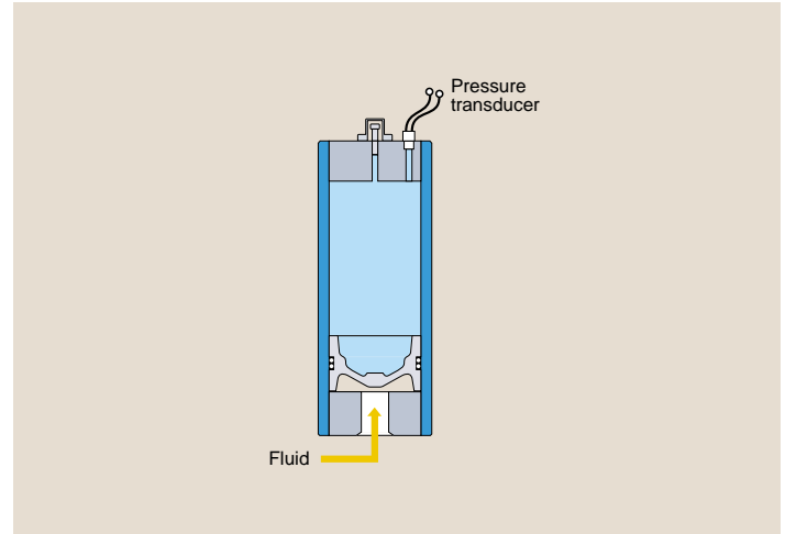
Fig. 14a Pressure transducer measures actual precharge pressure of shut down system
