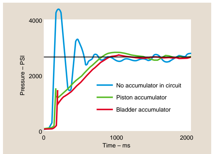
Fig.5 Shock wave test results - Example 2
