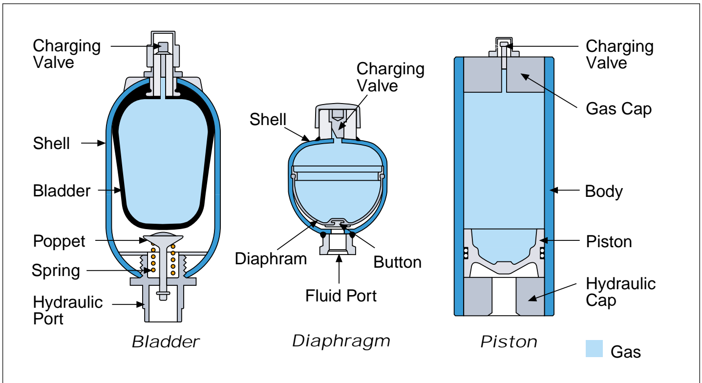
Fig.1 Typical bladder, diaphragm and piston accumulators
