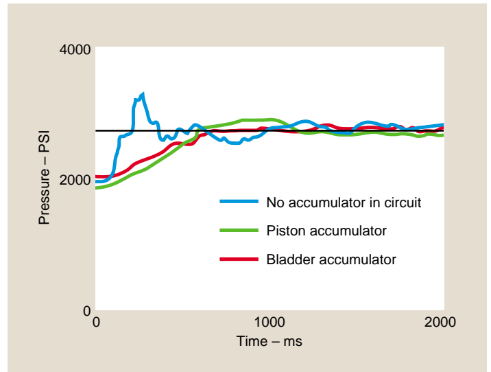
Fig.4 Shock wave test results - Example 1
