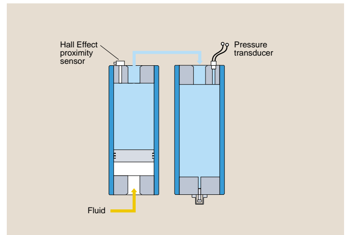
Fig. 14c Hall Effect sensor registers proximity of piston to end cap
