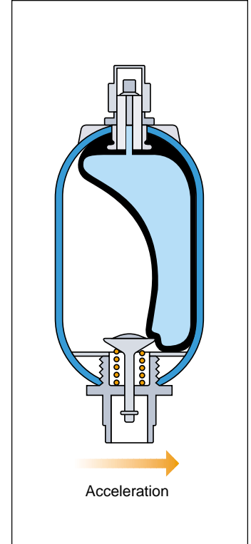
Fig.6 A horizontally-mounted bladder accumulator can trap fluid away from the hydraulic valve
