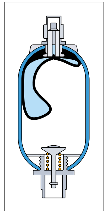
Fig. 13 Fluid entering an un-precharged bladder accumulator has forced the bladder into the gas stem
